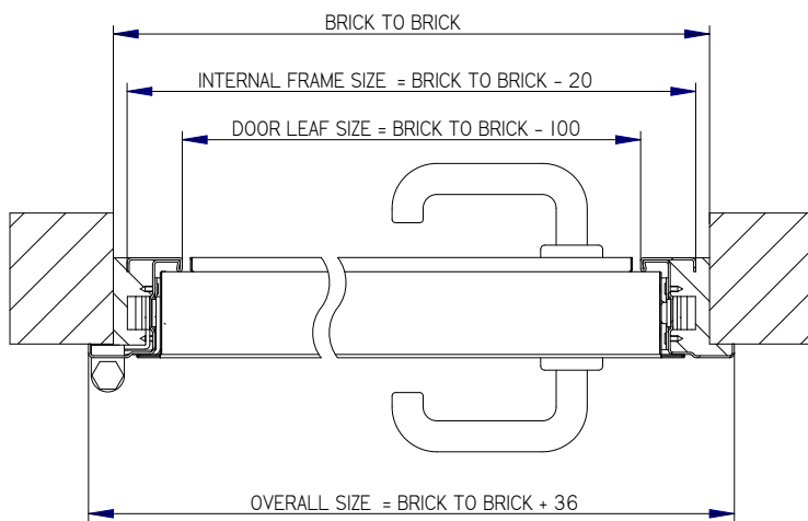
CROSS-SECTION B-B 1:6
