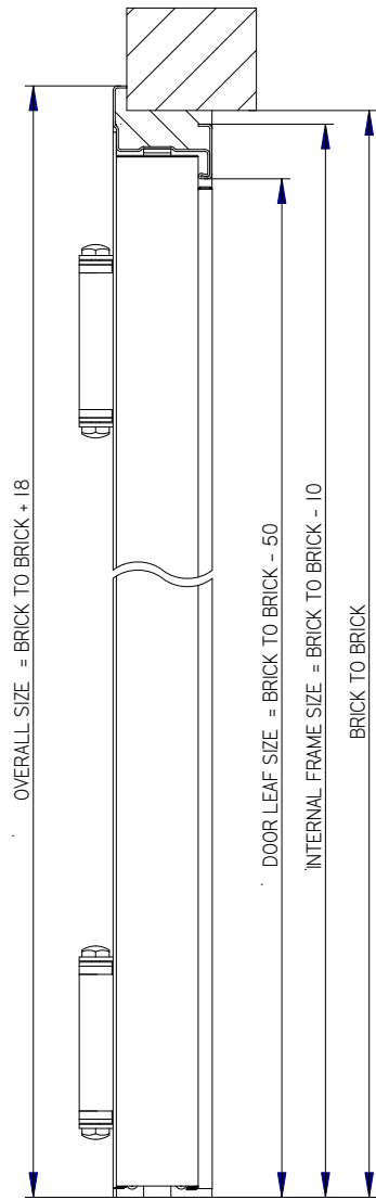
CROSS-SECTION A-A 1:6
