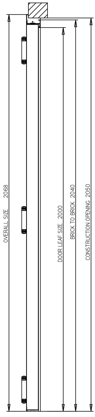
CROSS-SECTION A-A 1:5
