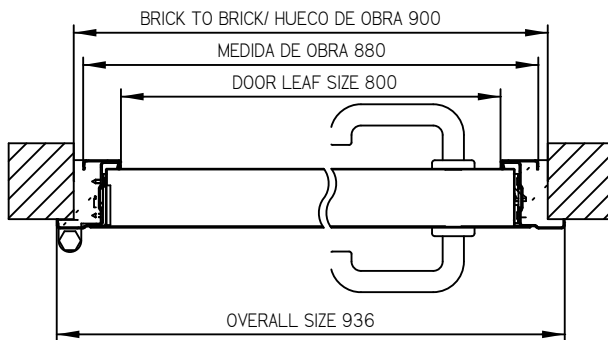
CROSS-SECTION B-B 1:8
