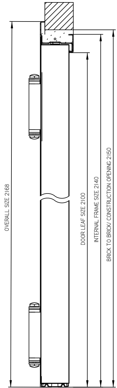
CROSS-SECTION A-A 1:5
